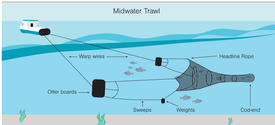
Figure 3. Midwater Pelagic Trawl
