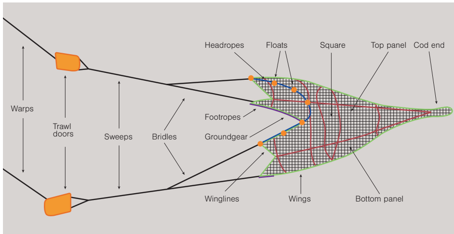
Figure 1. Overview of a trawl gear setup
